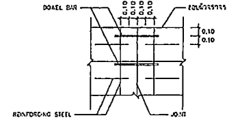
DETAIL B
